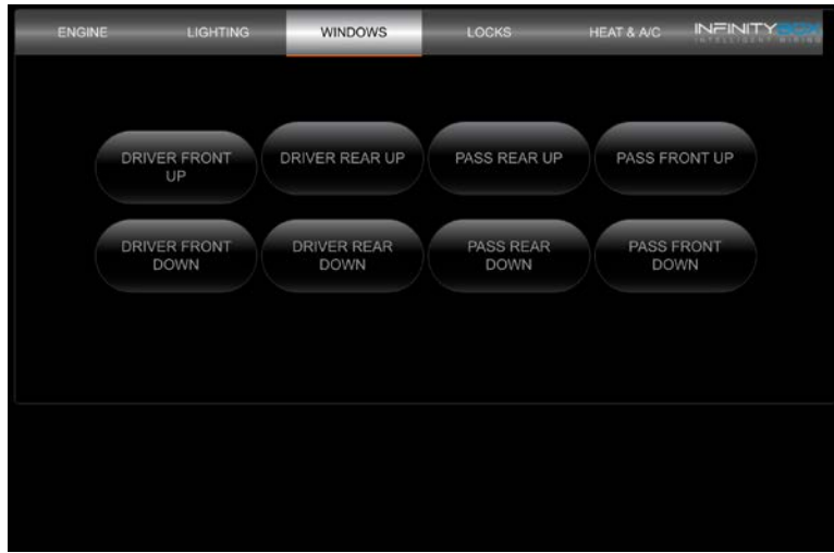
Figure 3: Windows Screen
